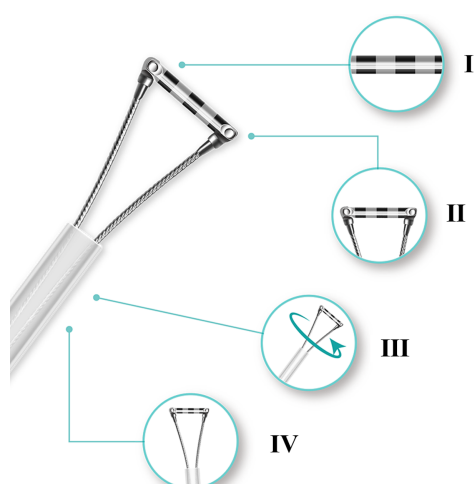
Figure 4 Diagram of improved Endoscopic Ruler. I: Clear scale; II: Shorter tip; III: Synchronous rotation; IV: More smooth edge.
