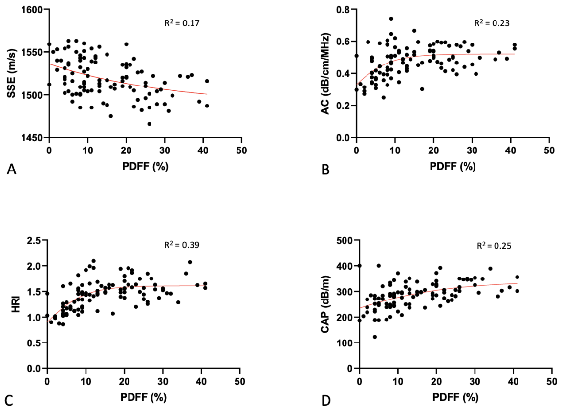
Supplementary figure 1 Scatterplots showing non-linear (logarithmic) relationship between SSE (A), AC (B), HRI (C) and cCAP (D) with MRI PDFF using 6-echo gradient. PDFF = proton density fat fraction, cCAP = continuous controlled attenuation parameter, SSE = sound speed estimation, AC = attenuation coefficient, HRI = hepatorenal index
