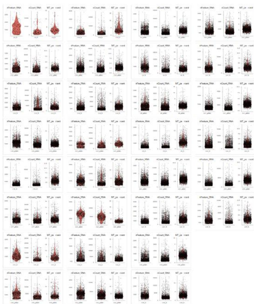
Supplementary Figure 1 Violin plots showing the result of quality control of each sample.
