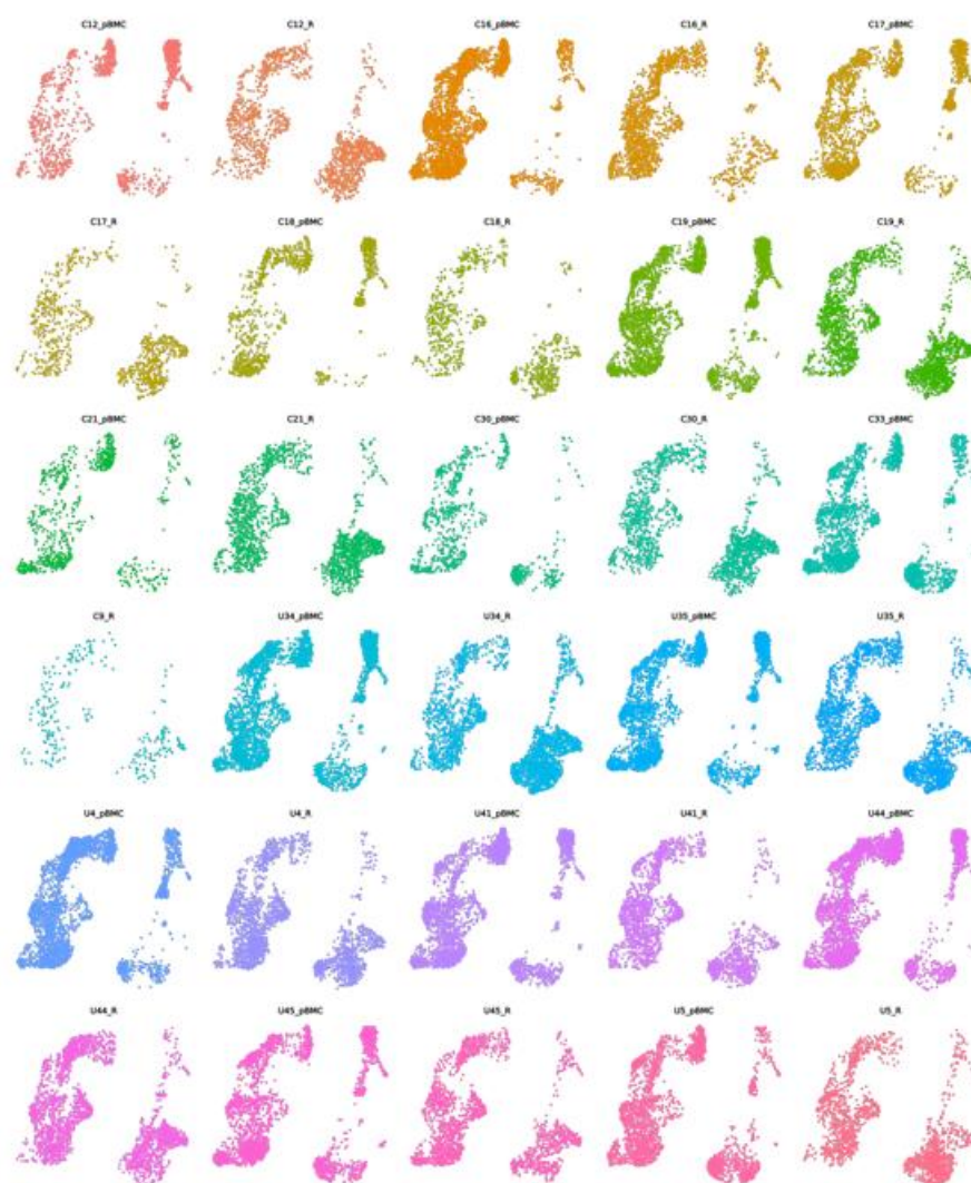
Supplementary Figure 2 Umap plots showing the cell distribution of each sample.
