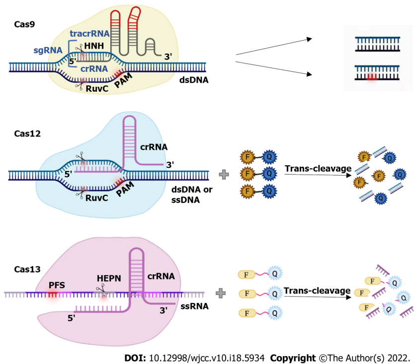
Figure 1 Collateral activity of Cas9, Cas12 and Cas13. PAM: Protospacer adjacent motif; dsDNA: Double-stranded DNA; ssDNA: Single-stranded DNA; crRNA: Clustered regularly interspaced short palindromic repeats RNAs; HEPN: Higher Eukaryotes and Prokaryotes Nucleotide-binding.
