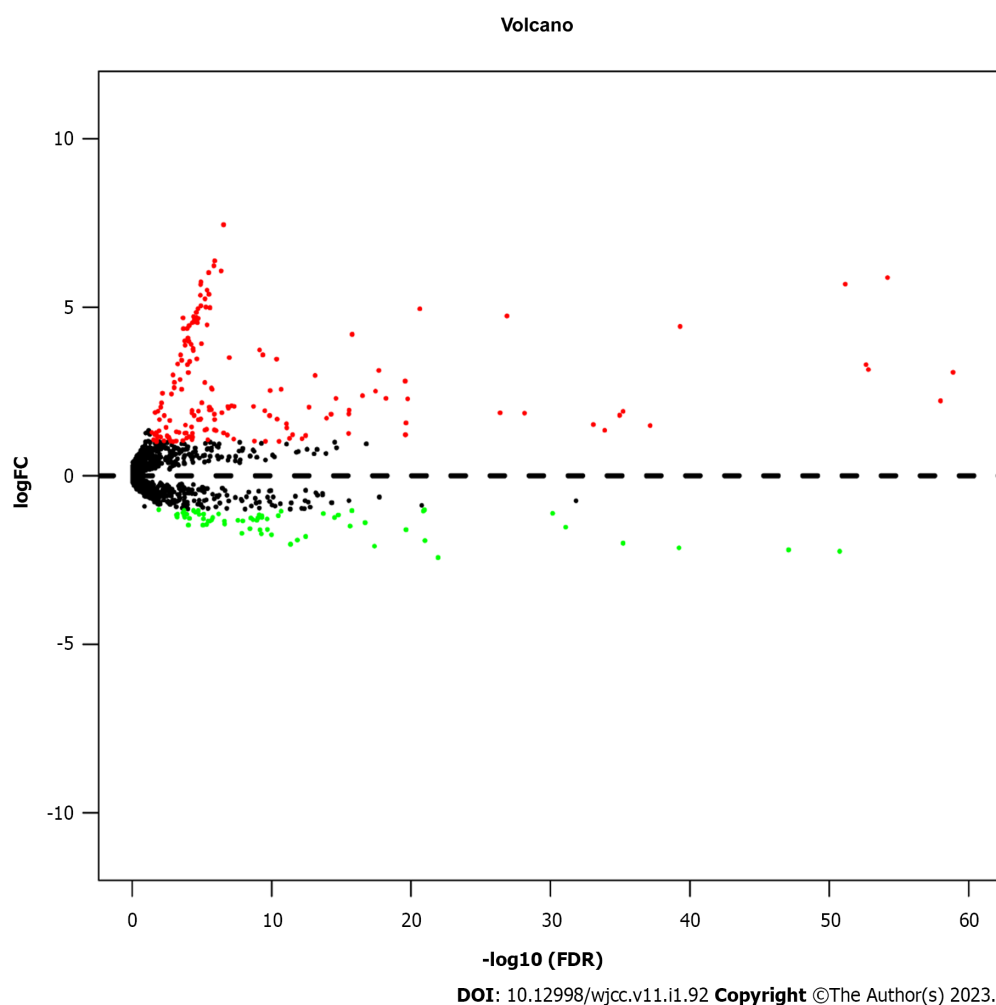
Figure 1 Volcano plot of 2202 miRNAs in papillary thyroid cancer patients. The red color indicates up-regulated expression, and the green color represents down-regulated expression. FDR: False discovery rate; FC: Fold change.
