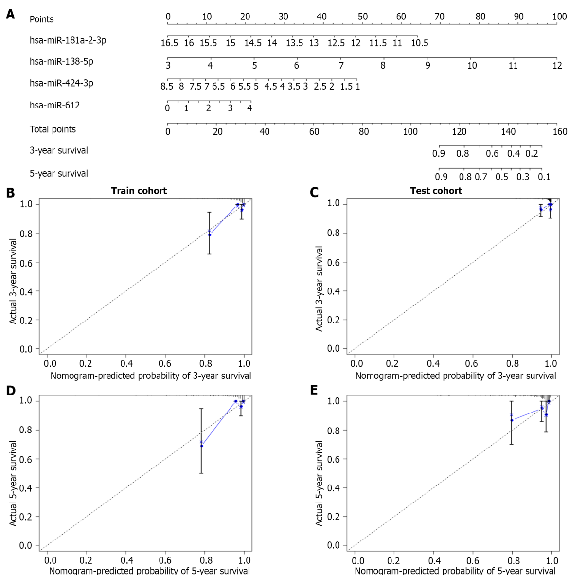
Figure 4 Prognostic nomogram and calibration plots of the four-miRNA signature. A: The prognostic nomogram based on the four-miRNA signature; B and C: Calibration plots of the four-miRNA-based prognostic model in the training and test cohorts of the 3-year survival rate; D and E: Calibration plots of the four-miRNA-based prognostic model in the training and test cohorts of the 5-year survival rate.
