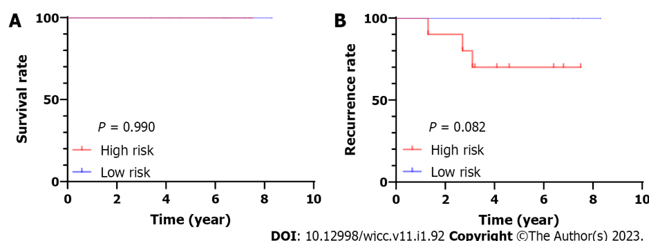
Figure 5 Validation the four-miRNA signature in transcriptome sequencing cohort. A: Overall survival curves; B: Recurrence-free survival curves in the whole-transcriptome sequencing cohort.
