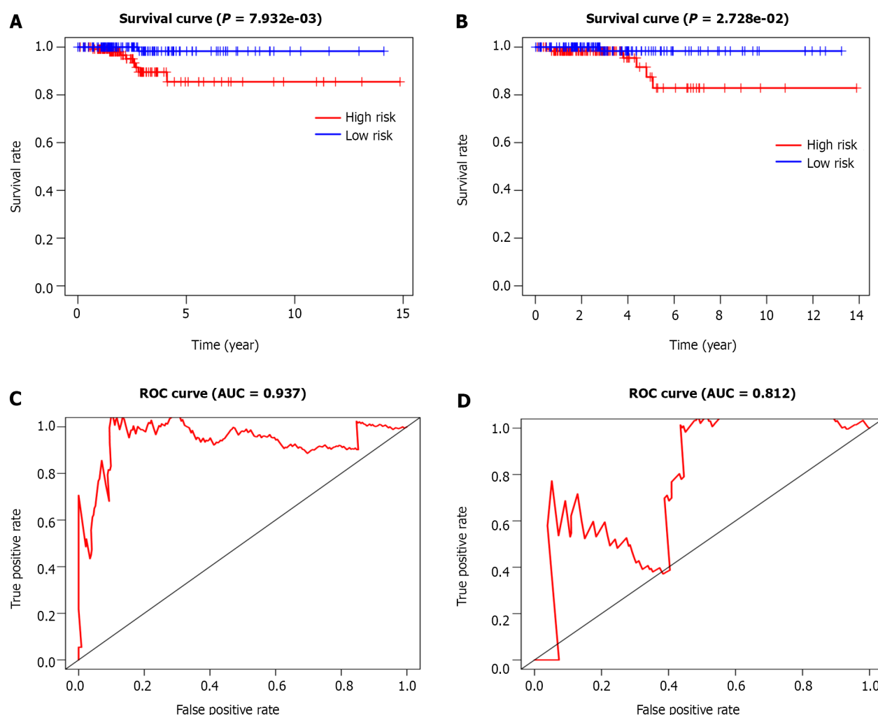
Figure 3 Kaplan-Meier curves of overall survival and time-dependent receiver operating characteristic curves of the 5-year survival rate for papillary thyroid cancer patients based on the four-miRNA signature. A and C: Training cohort; B and D: Test cohort. AUC: Area under the curve; ROC: Receiver operating characteristic.
