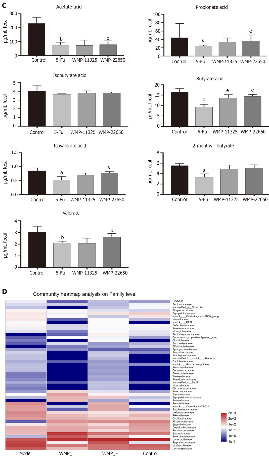
Figure 7 Effect of Wumei pills on taxonomy analysis of specific genera, the contents of short-chain fatty acids in feces, and heatmap of gut microbiota. A: Relative abundance of specific genera at each sample; B: Relative abundance of Lactobacillus , Bacteroides , Staphylococcus , Muribaculaceae ,
