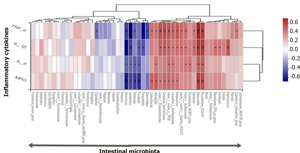
Figure 6 Kruskal-Wallis analysis of different bacterial groups, LEfse analysis, and microbiota-cytokine correlation. A: Phylum level; B: Class level; C: Order level; D: Family level; E: Genus level; F: Species level; G: Overall exhibition of LEfse analysis by cladogram; H: LDA scores of the specific enriched genera in each group; I: Spearman analysis of microbiota-cytokine correlation. WMP: Wumei pills; TNF- \alpha : Tumor necrosis factor- \alpha ; IL-6: Interleukin-6; IL-1 \beta : Interleukin-1 \beta ; MPO: Myeloperoxidase.
