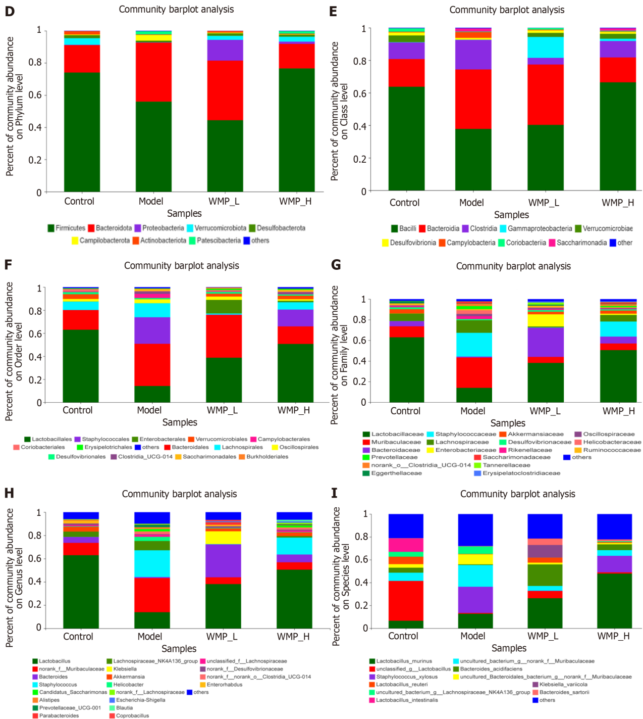
Figure 5 Microbial alpha, beta diversity, and taxonomy analysis. A: Dilution curve analysis; B: Alpha diversity (Shannon index, Simpson index, Ace index, and Chao index); C: Beta diversity; D-I: Taxonomy analysis of microbiota community. Values represent the mean \pm SEM. ^aP < 0.05 vs control group and ^bP < 0.05 , ^cP < 0.01 vs 5-Fu group. WMP: Wumei pills; 5-Fu: 5-fluorouracil.
