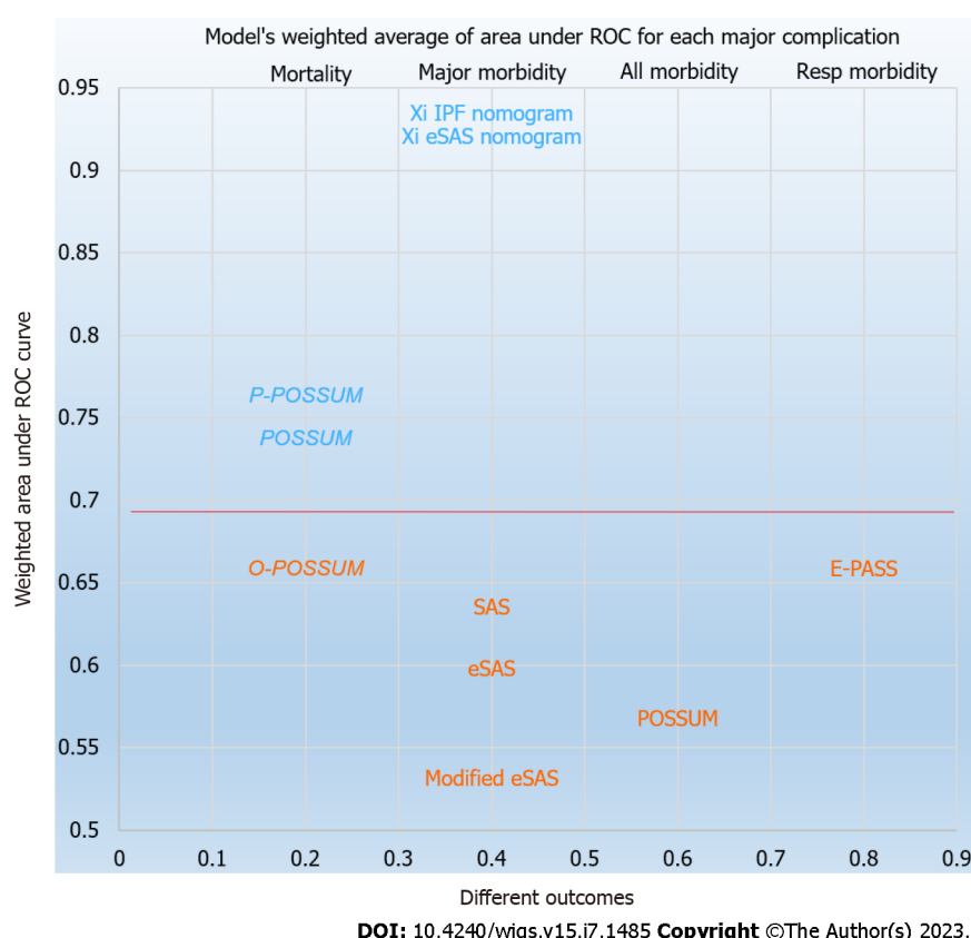
Figure 3 Weighted mean of c-statistics for each major outcome. ROC: Receiver operating characteristics; POSSUM: Physiological and operative severity score for the enumeration of mortality and morbidity; P-POSSUM: Portsmouth physiological and operative severity score for the enumeration of mortality and morbidity; O-POSSUM: Oesophagogastric physiological and operative severity score for the enumeration of mortality and morbidity; E-PASS: Estimation of physiologic ability and surgical stress; SAS: Surgical Apgar score; eSAS: Esophagectomy surgical Apgar score; IPF: Intraoperative factors.
