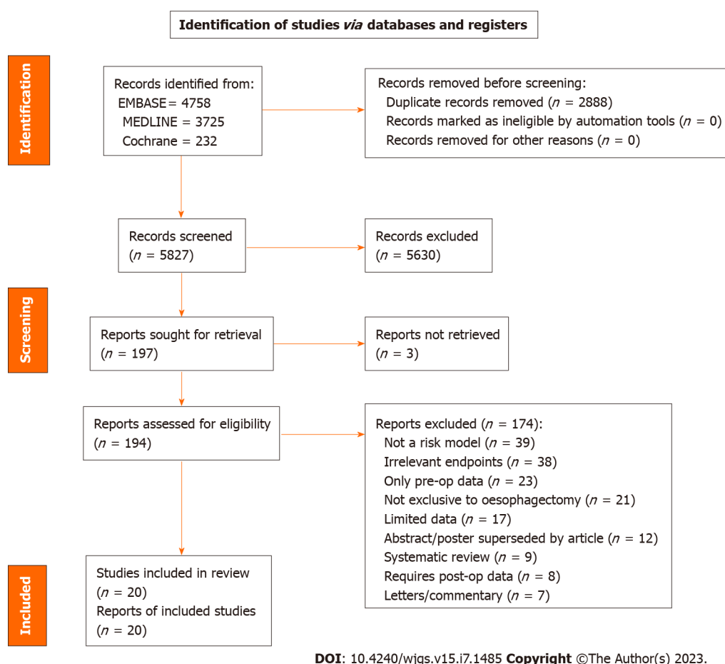
Figure 1 The preferred reporting items for systematic reviews and meta-analyses flow diagram of study selection.
