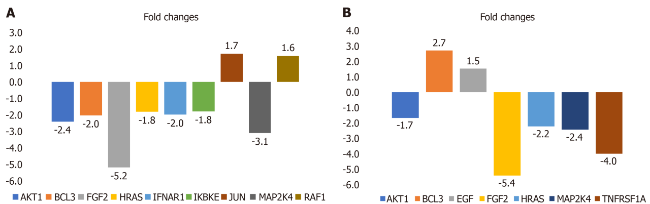
Figure 2 Significant gene expression. A: Significant gene expression in the post-laparoscopic anti-reflux surgery group compared to healthy controls; B: Significant gene expression in the post-laparoscopic anti-reflux surgery group compared to pre-laparoscopic anti-reflux surgery group. All comparisons are given as fold changes. BCL3: B-cell CLL/lymphoma 3; FGF2: Fibroblast growth factor 2; IFNAR1: Interferon (alpha, beta and omega) receptor 1; IKBKE: Inhibitor of kappa light polypeptide gene enhancer in B-cells, kinase epsilon; JUN: Jun proto-oncogene; MAP2K4: Mitogen-activated protein kinase 4; EGF: Epidermal growth factor; TNFRSF1A: Tumor necrosis factor receptor superfamily, member 1A.
