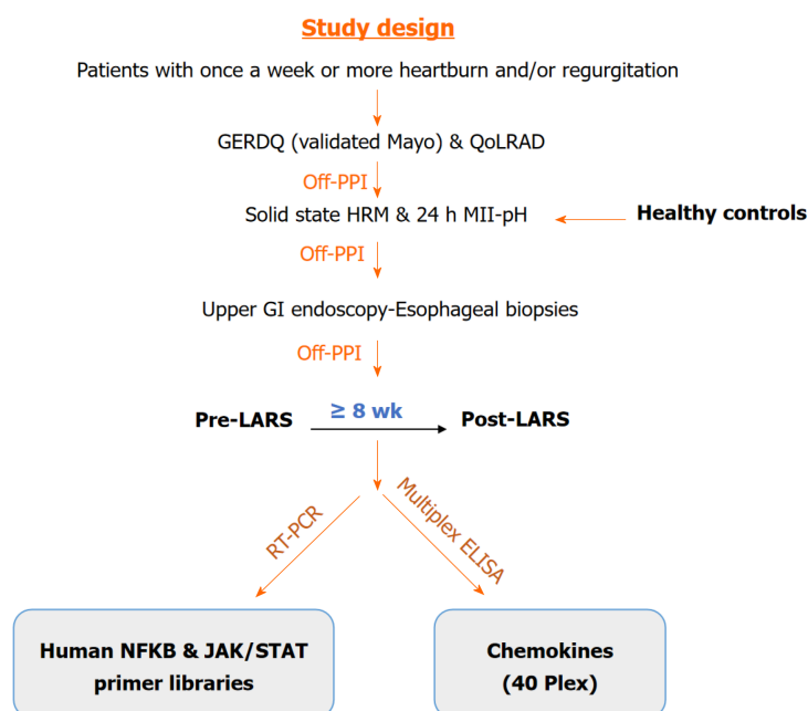
Figure 1 Study design. Pre-LARS: Pre-laparoscopic anti-reflux surgery; Post-LARS: Post-laparoscopic anti-reflux surgery; HRM: High-resolution manometry; MII-pH: Multichannel intraluminal impedance-pH; PPI: Proton pump inhibitor; RT-PCR: Real-time polymerase chain reaction; ELISA: Enzyme-linked immunosorbent assay; GI: Gastrointestinal.
