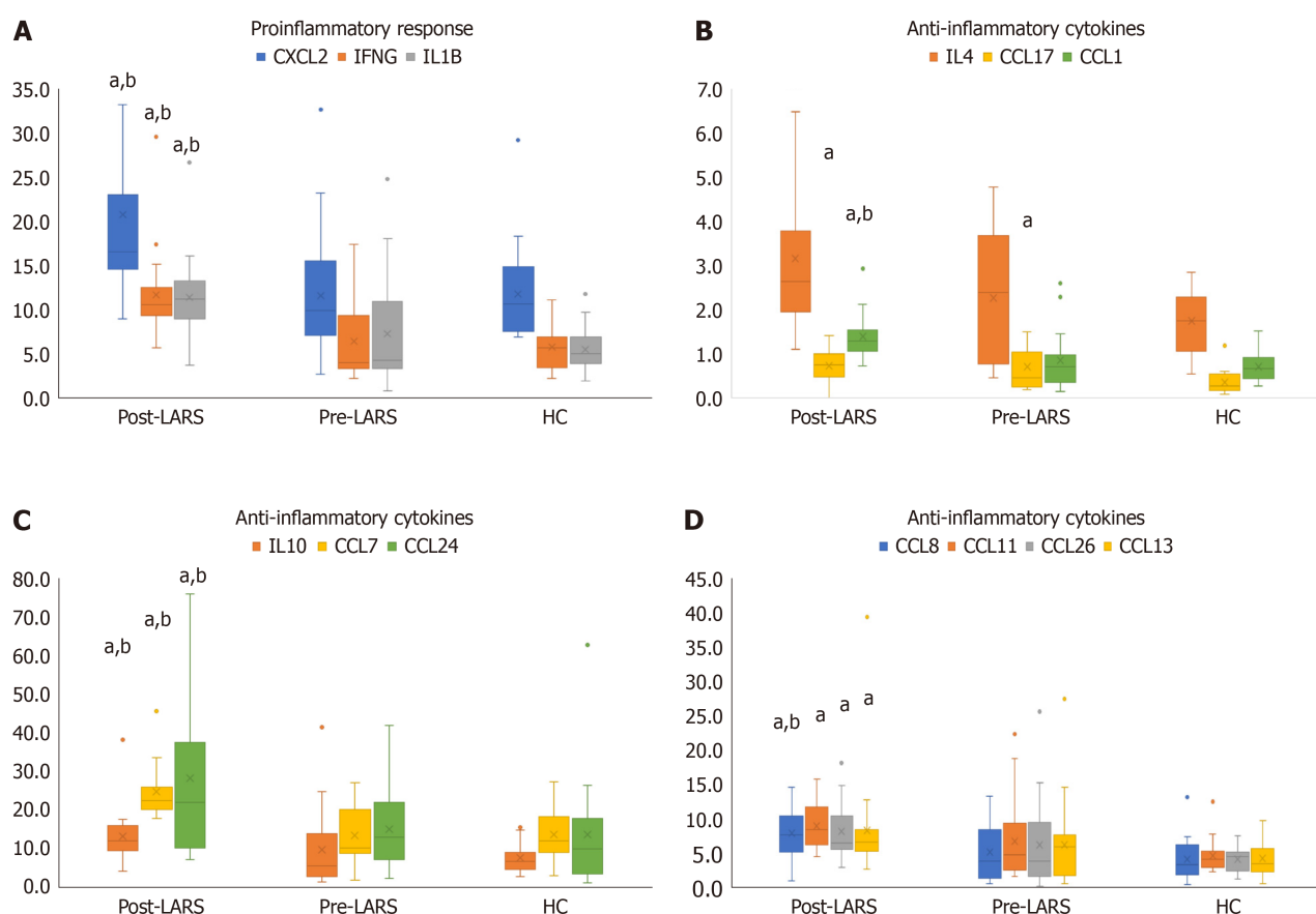
Figure 3 Cytokine results. A: Cytokine results indicating the proinflammatory response; B-D: Cytokine results indicating the anti-inflammatory response. a P < 0.05 vs healthy control; b P < 0.05 vs pre-laparoscopic anti-reflux surgery. CXCL: CXC motif chemokine ligand; IFN: Interferon gamma; IL: Interleukin; LARS: Laparoscopic anti-reflux surgery; HC: Healthy control.
