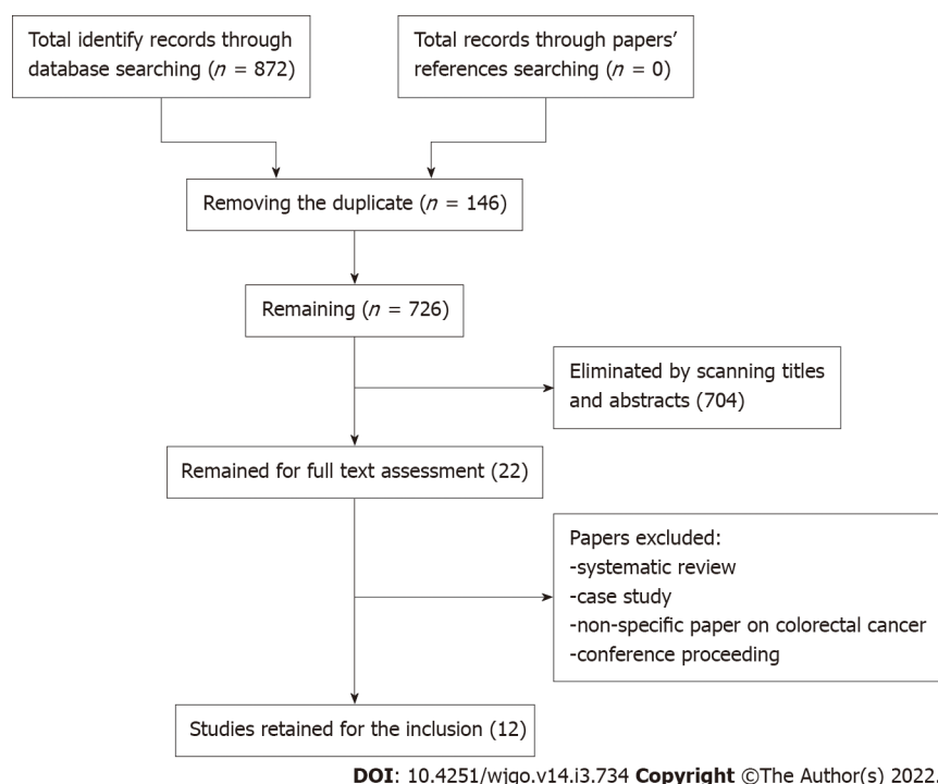
Figure 1 Search strategy.
