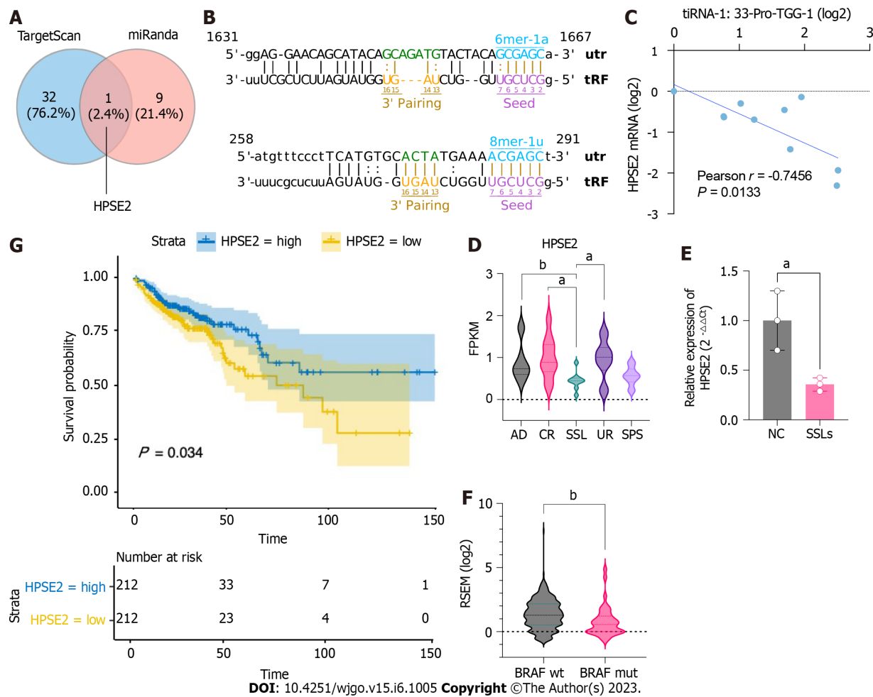
Figure 5 Potential target gene HPSE2 is involved in the serrated pathway. A: Schematic Venn diagram of transfer RNA halves (5'tiRNA)-Pro-TGG target gene prediction. B: Predicted interaction position between 5'tiRNA-Pro-TGG and 3'UTR of HPSE2 . C: Correlation analysis of the expression of 5'tiRNA-Pro-TGG and HPSE2 ( n = 10 ). D: Expression level of HPSE2 in common adenoma, right control colon tissue, sessile serrated lesion (SSL), right uninvolving colon, and serrated polyp syndrome in GSE76987. E: Expression level of HPSE2 in SSLs and normal control ( n = 3 ). F: HPSE2 expression in BRAF -mut colorectal cancer (CRC) was lower in BRAF -wild CRC. G: Kaplan-Meier survival curves for the overall survival (OS) of CRC patients in HPSE2 -high and HPSE2 -low groups. The OS of patients with HPSE2 -low was worse compared to that of patients with HPSE2 -high. a P < 0.05 , b P < 0.01 . AD: Common adenoma; CR: Right control colon tissue; SSL: Sessile serrated lesion; UR: Right uninvolving colon; SPS: Serrated polyp syndrome; OS: Overall survival; CRC: Colorectal cancer; NC: Normal control; tRF: Transfer RNA-related fragment; tiRNA: Transfer RNA halves.
