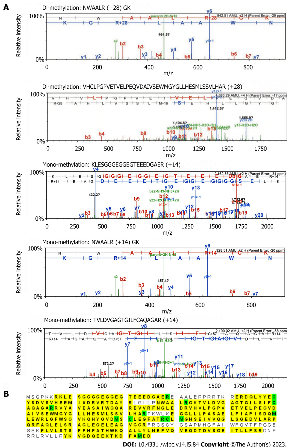
Figure 4 Liquid chromatography with tandem mass spectrometry analysis of the methylation sites on protein arginine methyltransferase
