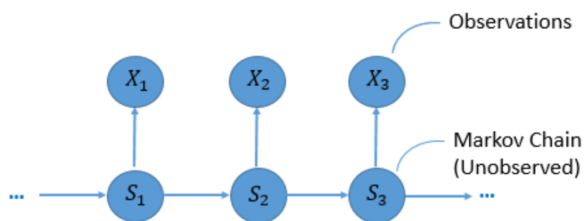
Supplementary Figure 1 Hidden Markov Model [121] .
