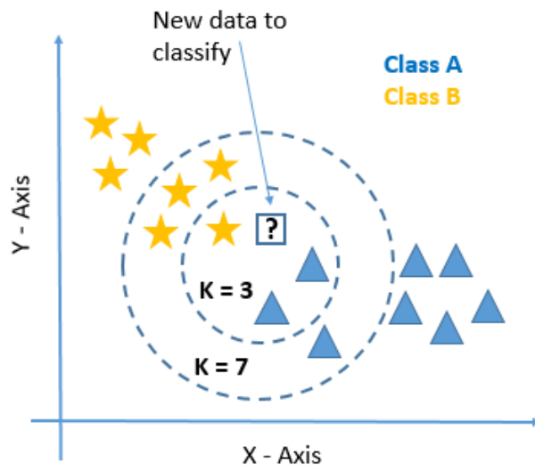
Supplementary Figure 3 K-Nearest Neighbor Algorithm [123] .
